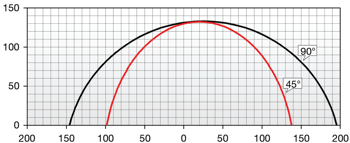
Cutting chart
