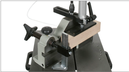
Clamps 02
